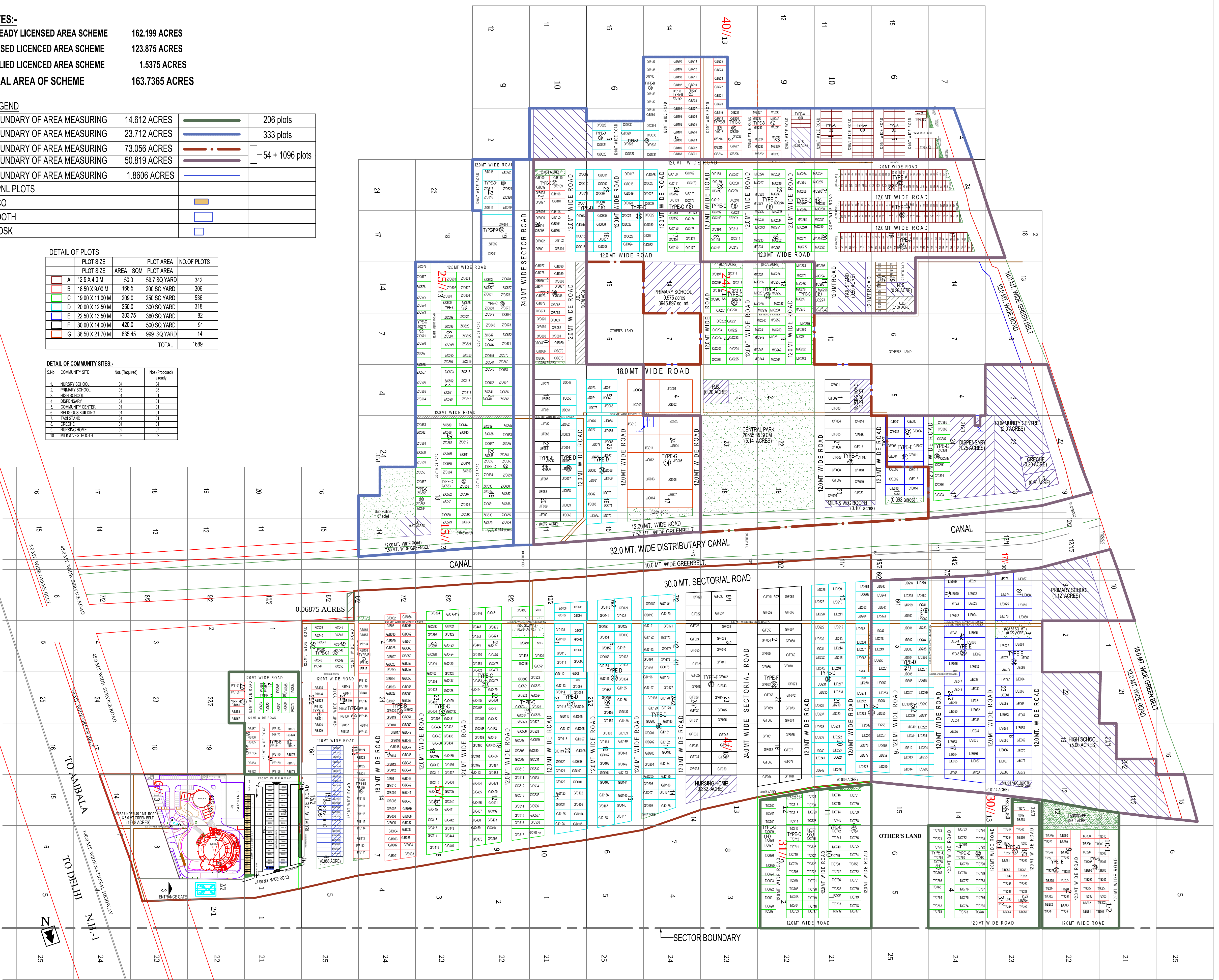
CHD CITY, LAYOUT AREA =163.7365 ACRES
